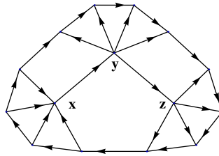
Fig. 2. An oriented leaf distant Halin graph for which \bar{\lambda} = 7 .
