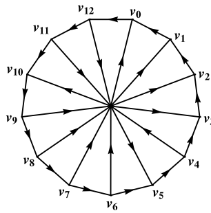
Fig. 1. An oriented wheel \vec{W} for which \vec{\lambda}(\vec{W}) = 8 .
