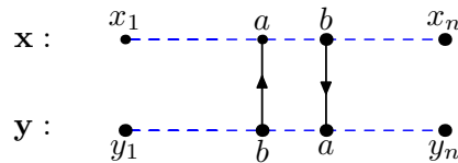
Figure 3.1: The edge \{a, b\} appears in both directions.
