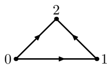
(a) \Sigma(T_3) = \log 3
