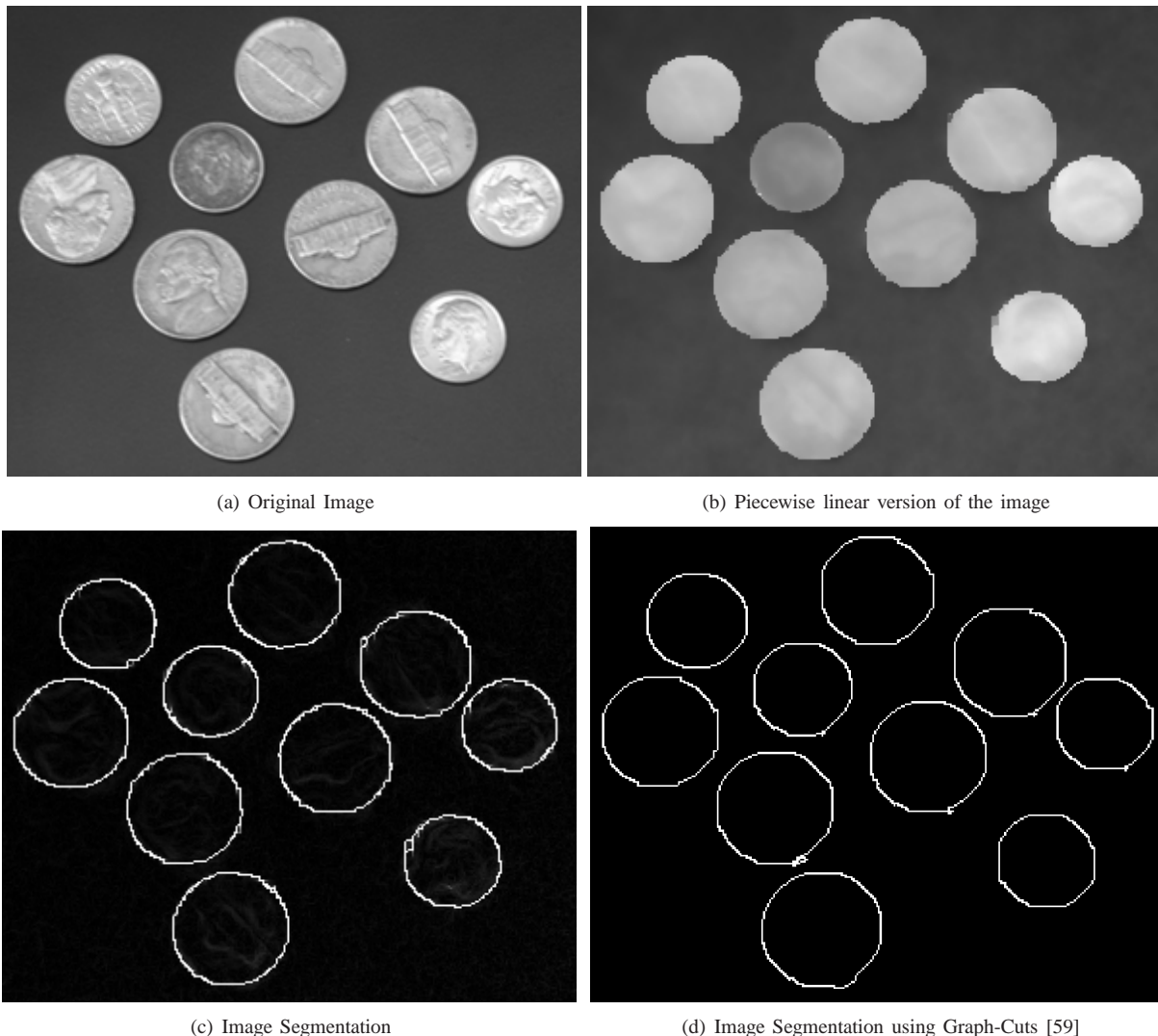
Fig. 9. Piecewise linear version of coins image together with the segmentation result. We compare to the popular graph-cuts based segmentation [59].
