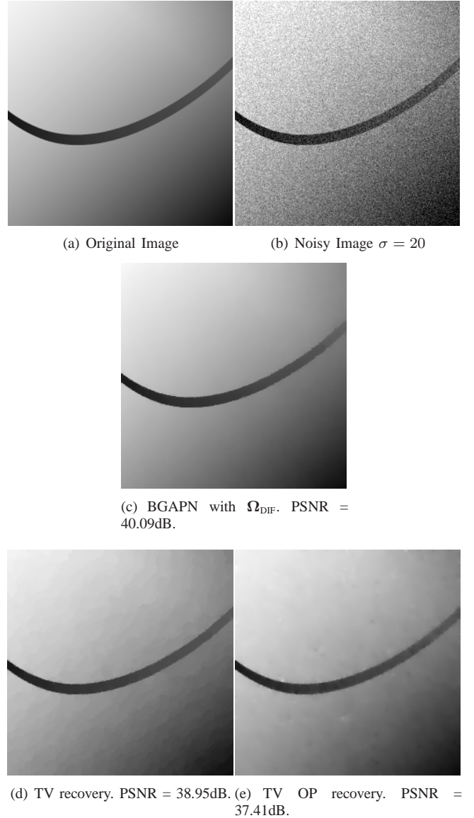
Fig. 5. Denoising of swoosh using the BGAPN algorithm with and without diagonal derivatives. Notice that we do not have the staircasing effect that appears in the TV reconstruction.
