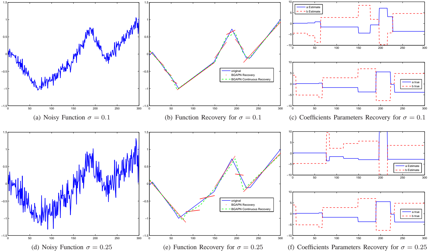
Fig. 1. Recovery of a piecewise linear function using the BGAPN algorithm with and without a constraint on the continuity.
