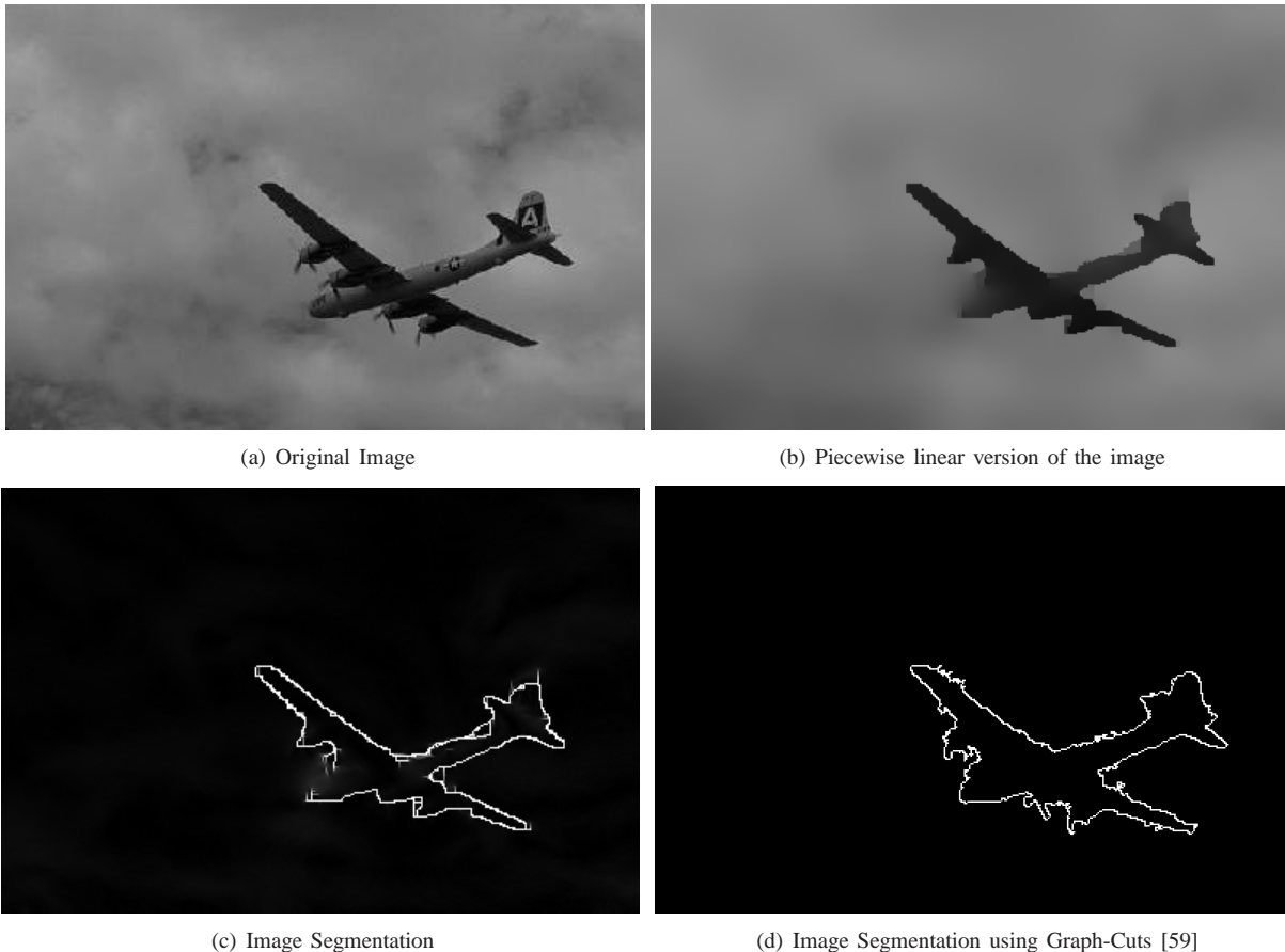
Fig. 10. Piecewise linear version of airplane image together with the segmentation result. We compare to the popular graph-cuts based segmentation [59].
