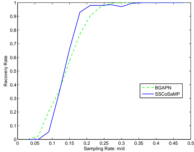
Fig. 4. Recovery rate of piecewise second-order polynomial functions as a function of the sampling rate m/d for the methods BGAPN and SSCoSAMP.
