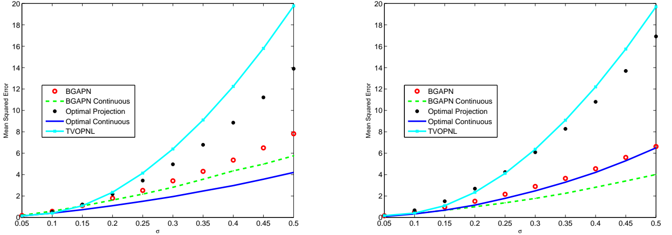
Fig. 3. MSE of the recovered piecewise linear functions (left) and piecewise second-order polynomial functions (right) as a function of the noise variance \sigma for the methods BGAPN with and without the continuity constraint and the optimal approximation with and without continuity post-processing. As a reference we compare to the non local overparameterized TV (TVOPNL) approach introduced in [38].
