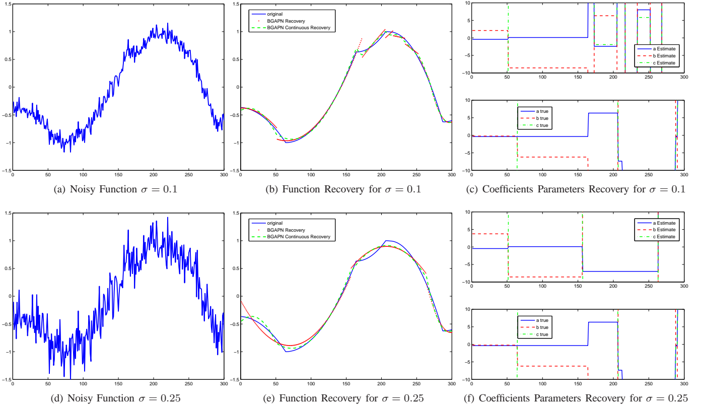
Fig. 2. Recovery of a piecewise second-order polynomial function using the BGAPN algorithm with and without a constraint on the continuity.
