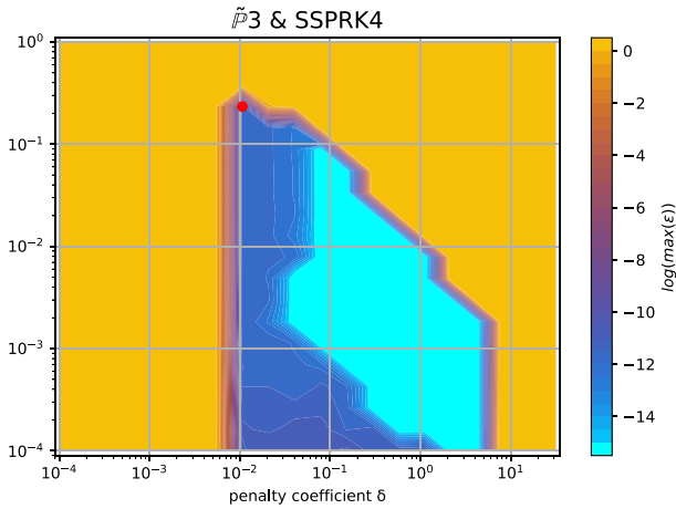
Fig. 13 Logarithm of the amplification coefficient \log(\max_i(\epsilon_i)) for SUPG stabilization with \tilde{\mathbb{P}}_3 Cubature elements and the SSPRK method. Unstable region in yellow, the red dot is the optimal parameter according to (50)
