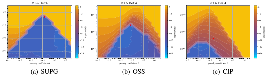
Fig. 8 Damping coefficients \log(\max_i \epsilon_i) for \mathbb{B}_3 Bernstein elements and the DeC method with, from left to right, SUPG, OSS and CIP stabilization. The red dot is the optimum according to (50)
